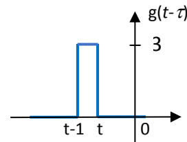
Fig 6. Translation de g(\tau)
